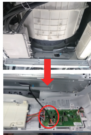
Connecting connector MAIN PWB~ Display PWB
