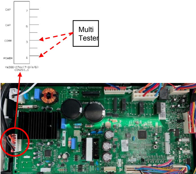
A-Inverter
